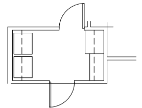
OPT. UTILITY CABINETS
