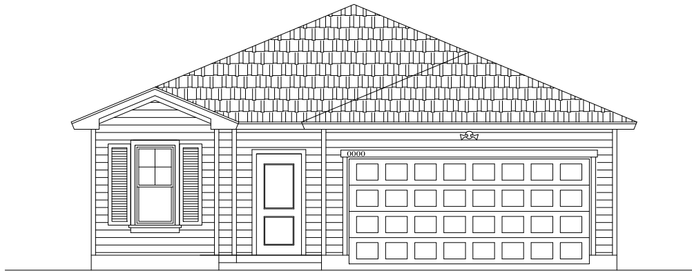
ELEVATION C
