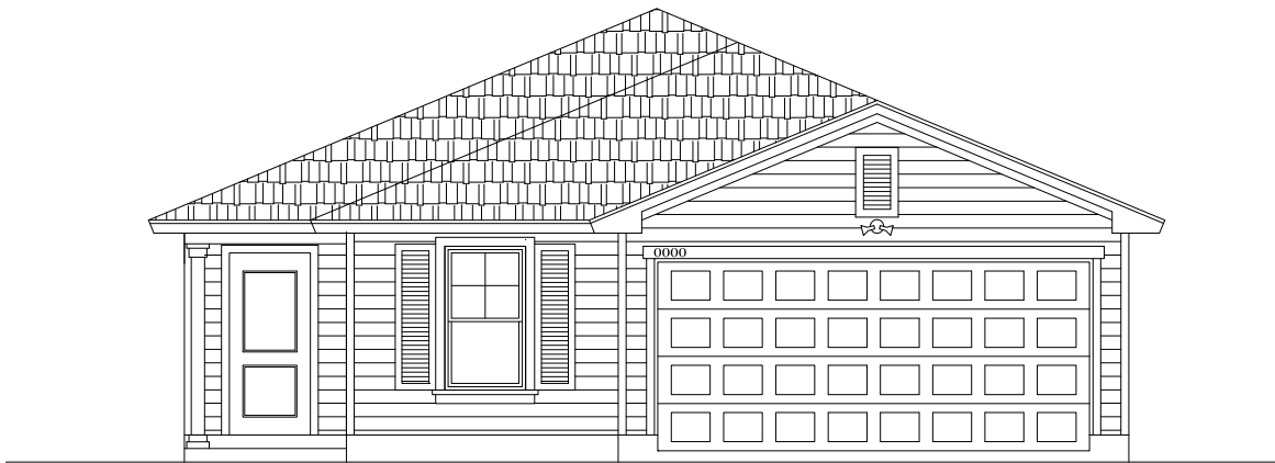
ELEVATION C
