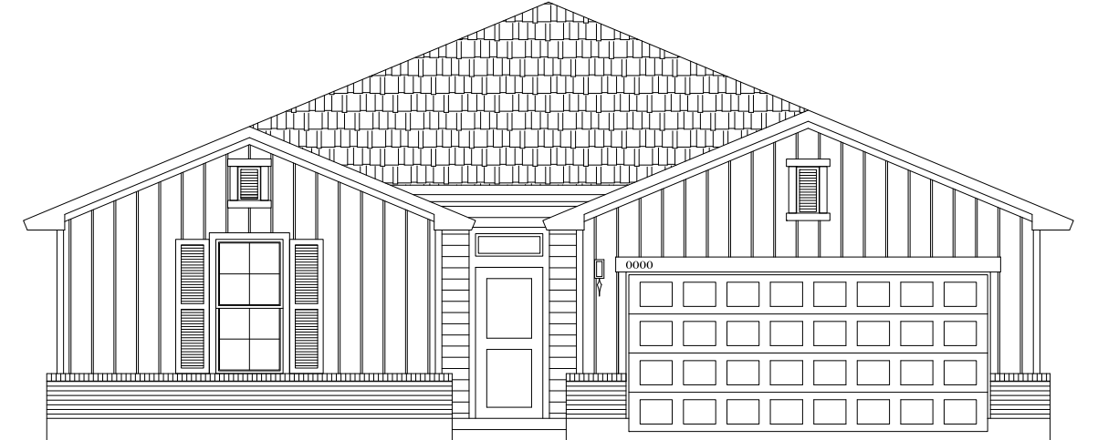
ELEVATION W
