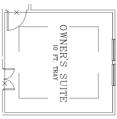
OWNER'S SUITE 10 FT. TRAY OPTIONAL TRAY CEILING
