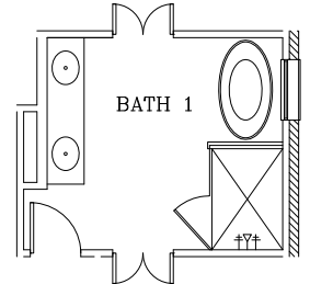
BATH 1 FREESTANDING TUB
