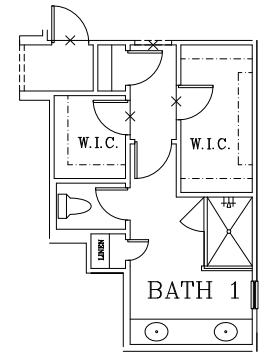
BATH 1 SHOWER OPTION 1
