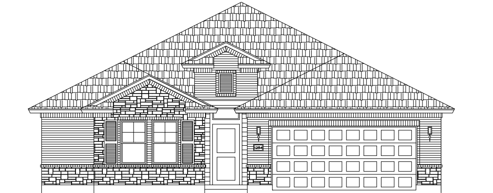
ELEVATION A – STONE UPGRADE
