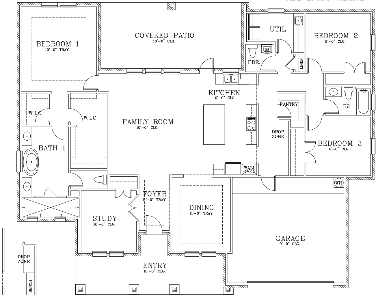
SIDE ENTRY GARAGE
