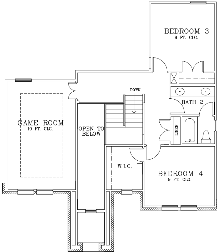
SECOND FLOOR WITH GAME ROOM
