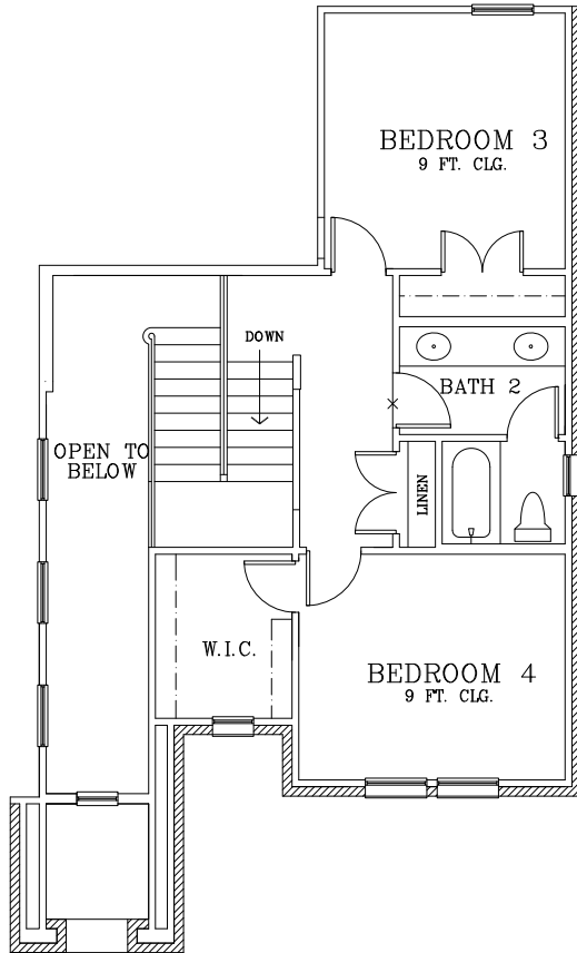
STANDARD SECOND FLOOR
