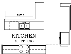
BANQUETTE KITCHEN ISLAND
