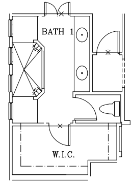
BATH 1 WALK IN SHOWER OPTION OPTION 2
